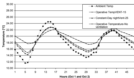
Figure 5: Influence of different ventilation strategies
